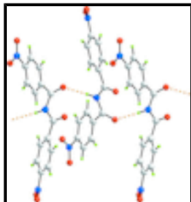
Fig. 2. Supramolecular chain aligned along the b axis in (I) mediated by N—H...O hydrogen bonding shown as orange dashed lines.
